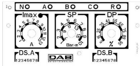
Figure 16: Regulating: I_{max} , SP and DP
