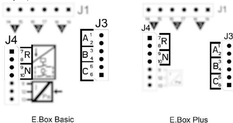
Figure 44: Inputs
