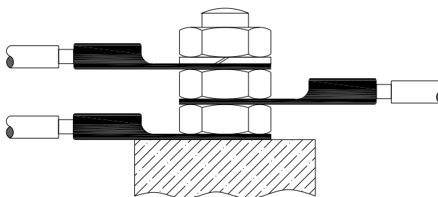
Figure 2: Earth connection
