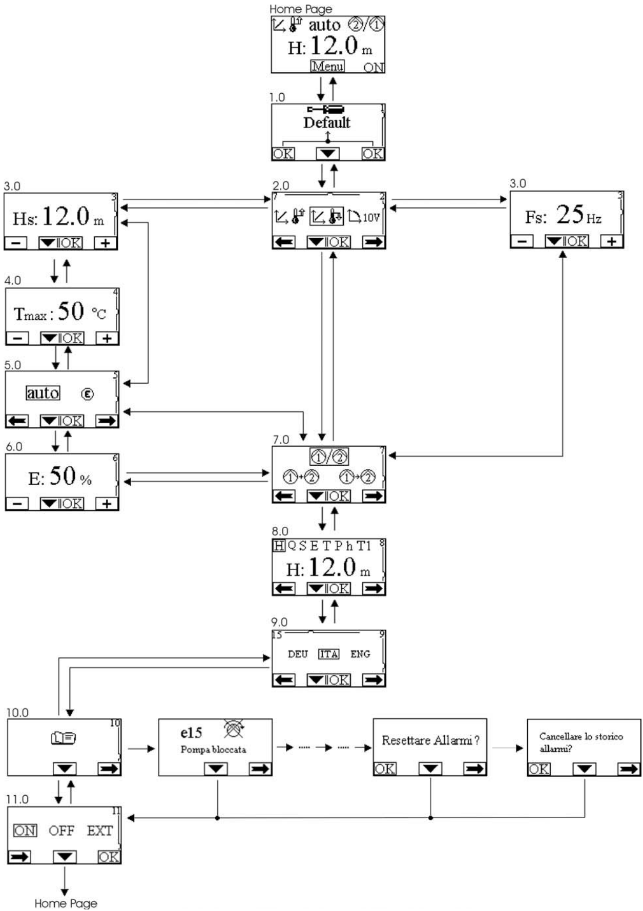
Figure 8: MCE/C Menu
